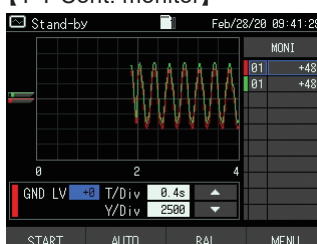
Y-T graph display (continuous display)
