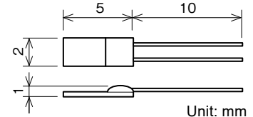
External dimensions
