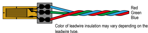
TFL (Connecting terminal joint type) -6FB□LT(CT)
