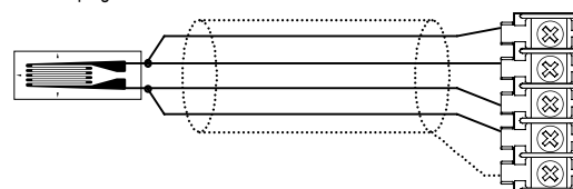
Built-in switching box of data logger TDS-540 is not applicable
