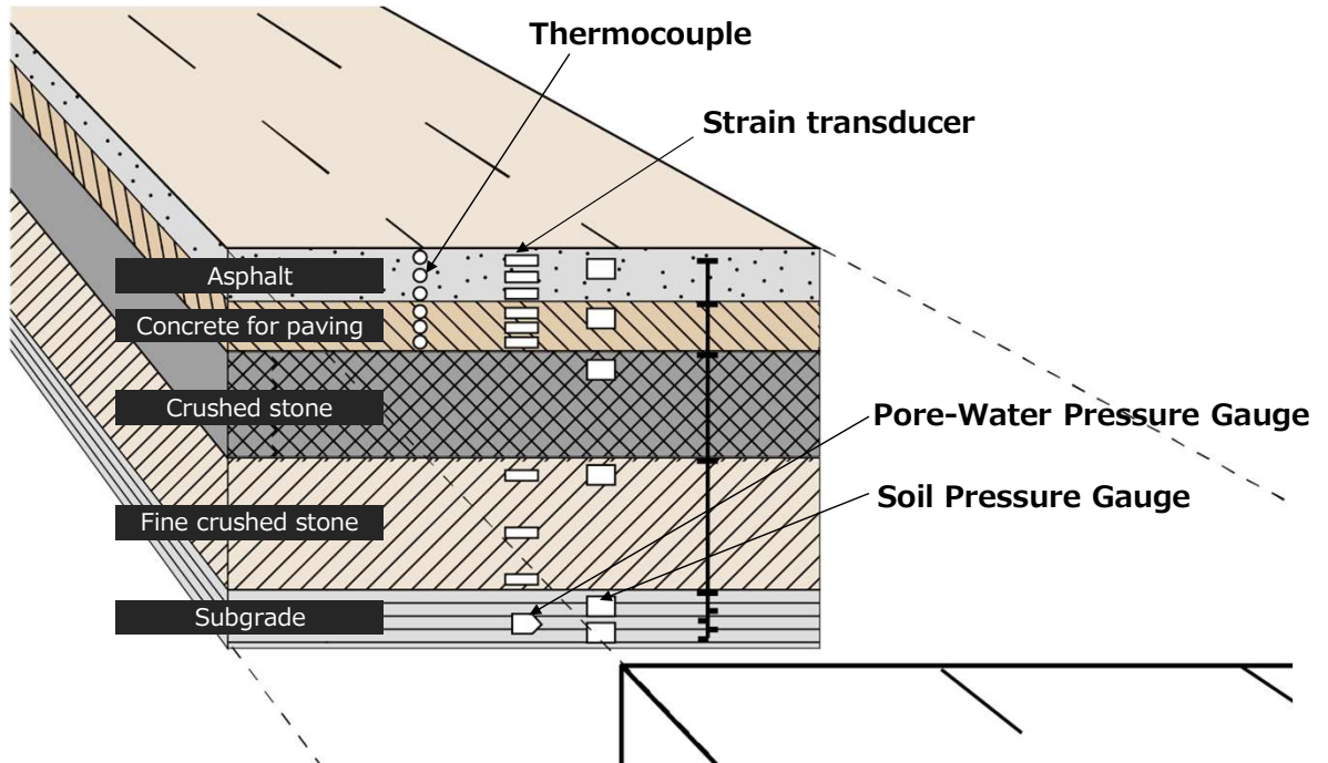
[ Measuring System Block Diagram ]
