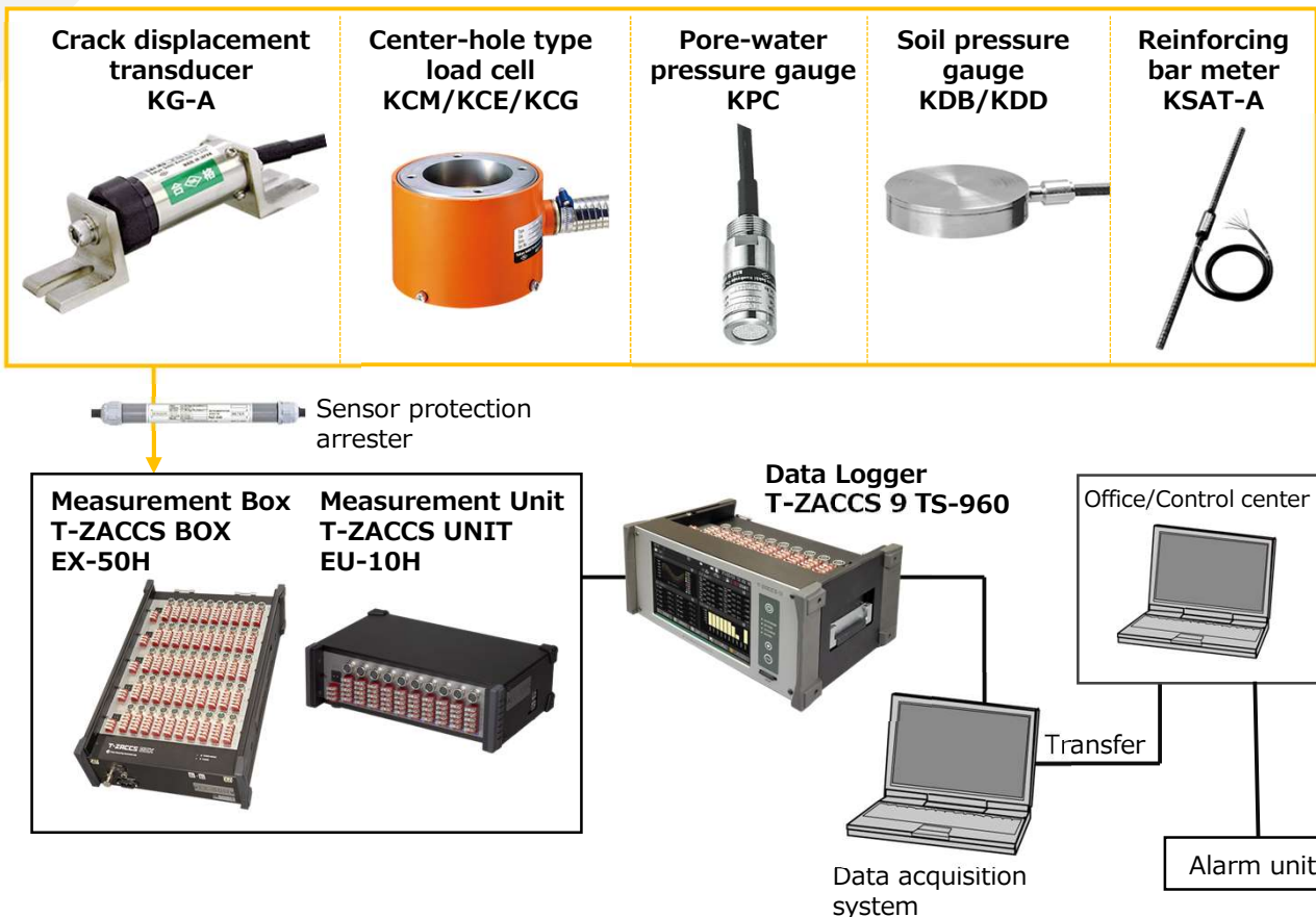
[ Measuring System Block Diagram ]
