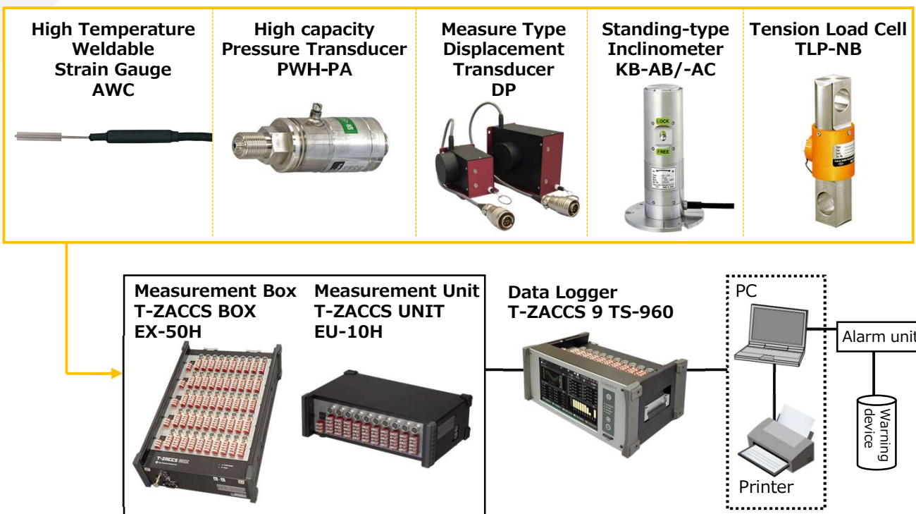
[ Measuring System Block Diagram ]
